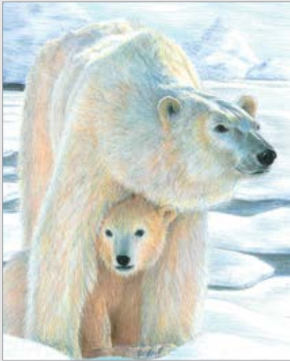
CPN22 Polar Love UPC: 090672 373656
